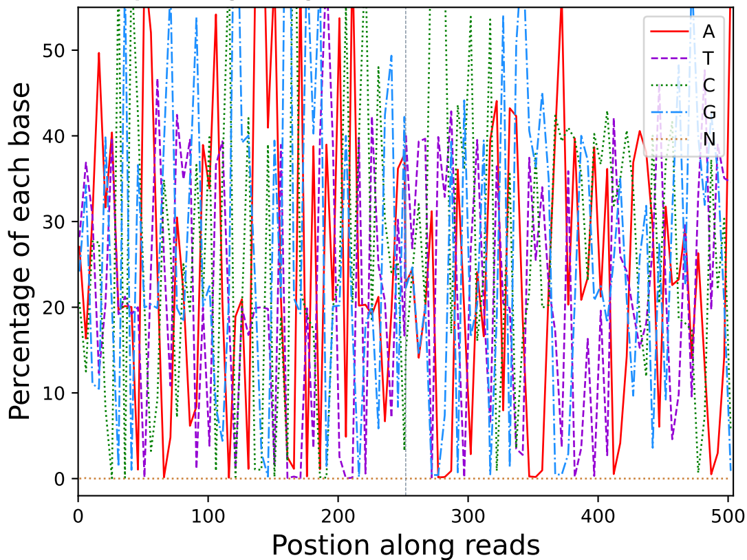
Base percentage along reads (R10419)
